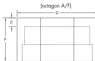
Insulating cap
